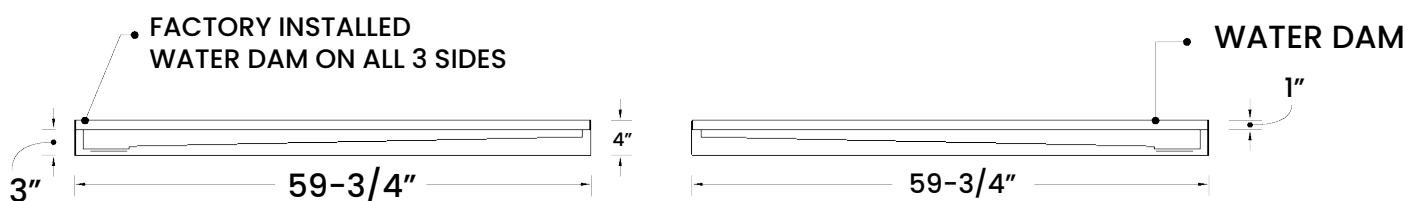
Front View
